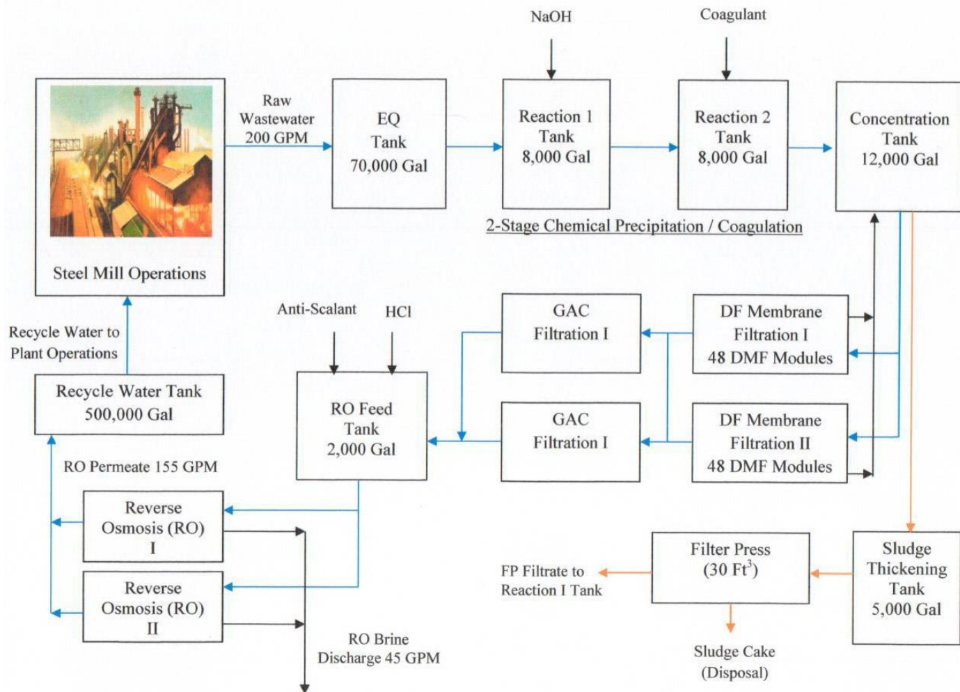
Figure 3: Full Scale installation Schematic
