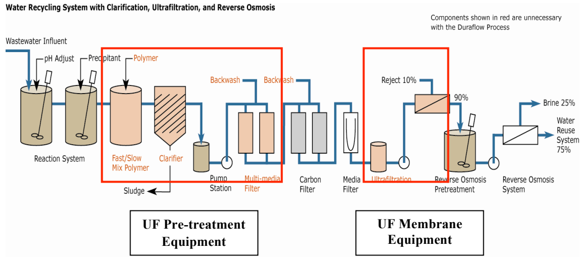
Figure 2 - Typical Duraflow MF/RO Water Recycle Process Configuration
